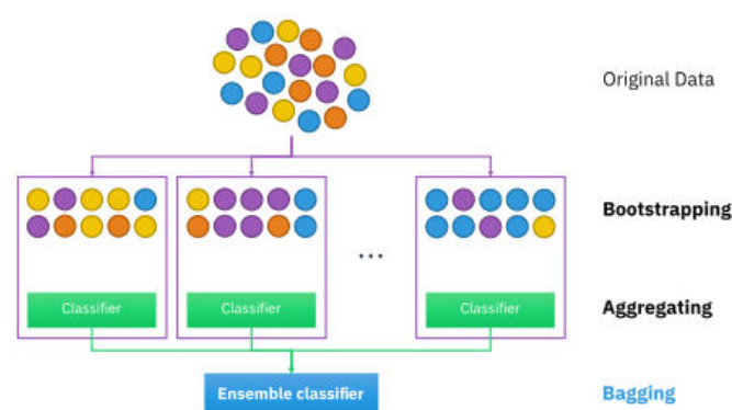
Figure3.2: RF Classifier analysis.
