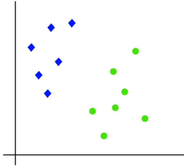
Figure 3.6: Linear SVM
