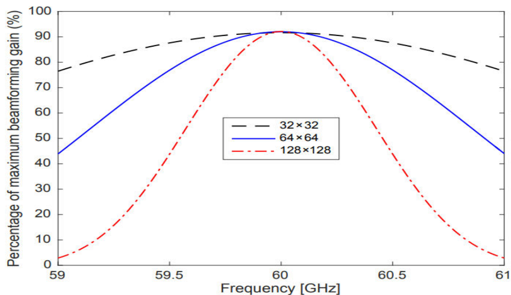
Figure 4. The fraction of the maximum beamforming gain that is achieved at different frequencies when analog beamforming is used.
