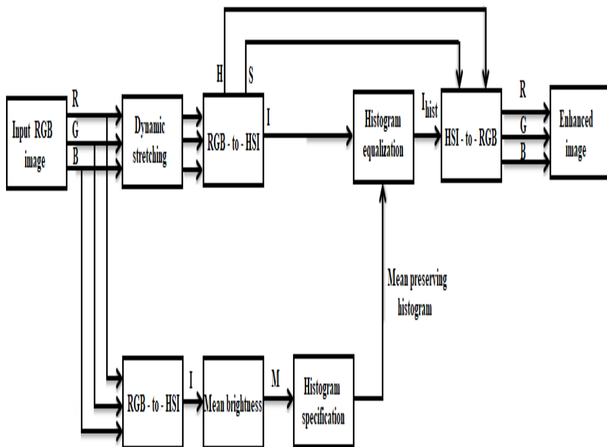
Figure 1: Proposed block diagram for brightness preserving histogram equalization approach.
