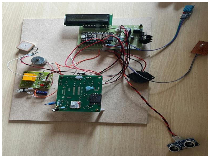
Figure:2: iot-based intelligent systems for road saftey using vehicle-to-interface (v2i) system
