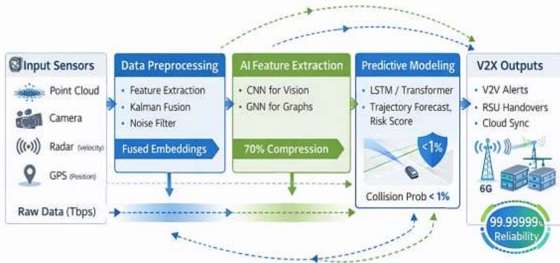
Figure 2: AI pipeline for predictive V2X communications
